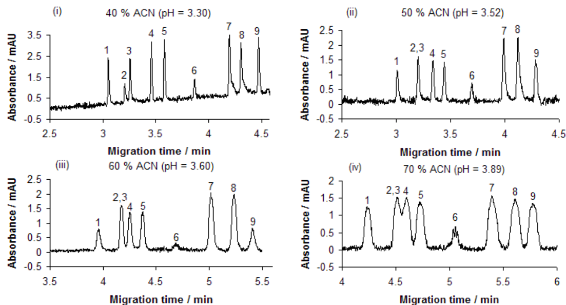
Fig. 3: Electropherograms of peptide mixture in 0.5 % FA + 10 mM TEA + different amounts of ACN (40 - 70 %). Voltage: 30 kv (i) – (ii), 25 kv (iii) 20 kv (iv). Other experimental details are similar to Fig. 1.
