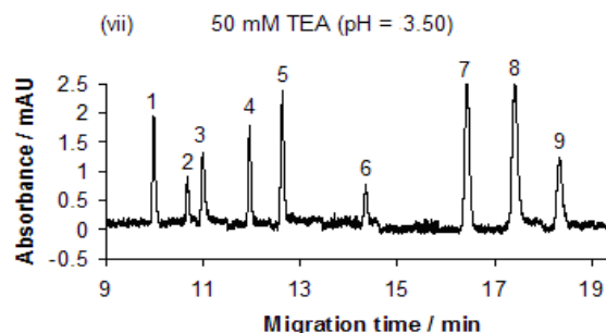
Fig. 2: Electropherograms of the peptides mixture in 1.0 % FA + 30 % ACN + different concentrations (0 - 50 mM) of TEA at respective pH. Sample conc.: 5.0 \text{ ng } \mu\text{L}^{-1} , voltage: 25 kv (i) – (iii) & (v), 20 kv (iv), 15 kv (vii), 10 kv (vi). Other experimental details are similar to Fig 1.
