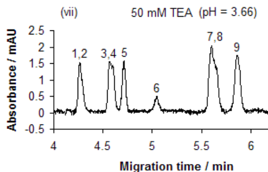
Fig. 1: Electropherograms of the peptides mixture in 0.5 % FA + 30 % ACN + different concentrations (0 - 50 mM) of TEA, at respective measured pH. Sample conc.: 0.65 - 2.5 \text{ ng } \mu\text{l}^{-1} , voltage: 30 kv (i) – (iv), 25 kv (v) – (vii); data rate: 16 Hz; and UV detection at 190 nm. Peaks identification: 1 – bradykinin; 2 – substance P; 3 – bradykinin F1-5; 4 – Arg 8 -vasopressin; 5 – LHRH; 6 – bombesin; 7 – Leu-enkephalin; 8 – Met-enkephalin; 9 – oxytocin.
